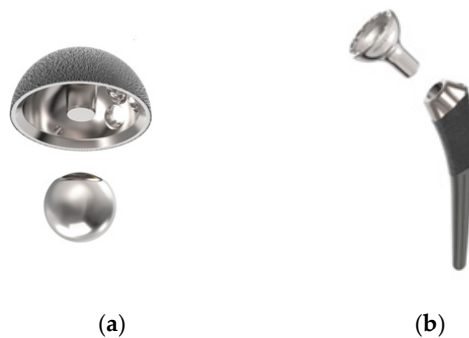
Figure 3. Tapers visually evaluated for corrosion: Acetabular Taper (a) and Femoral Taper (b).
